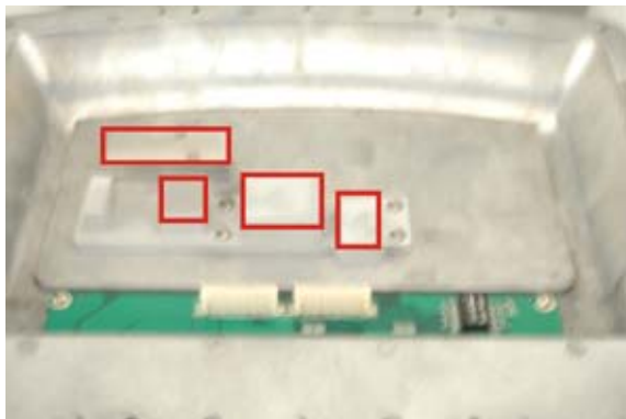
Figure 6-4: Thermal Pads
