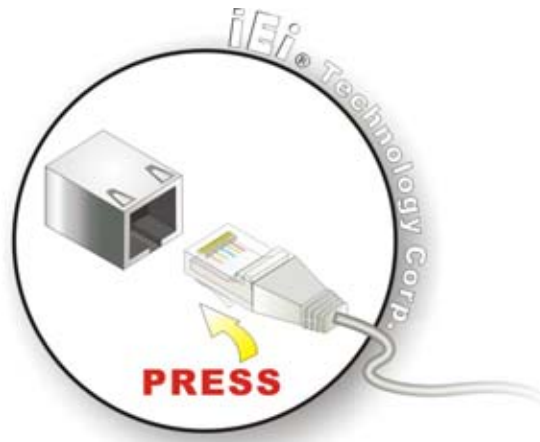
Figure 3-13: LAN Connection
