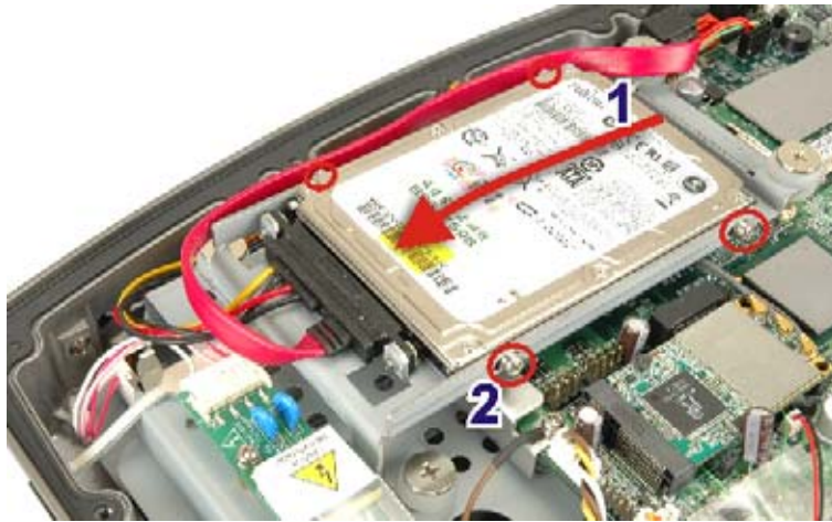
Figure 3-3: HDD Installation
